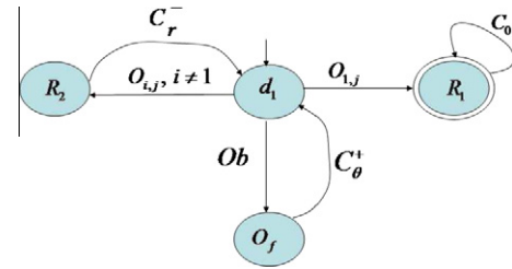
Fig. 20. The refined closed loop system automaton G_{clref} , where G_{clref} = S || G_{ref} and S = S_f || S_{Ca} .
