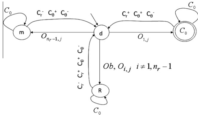
Fig. 17. Modified DES model of the plant.
