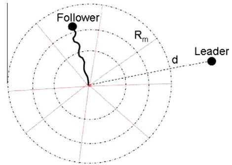
Fig. 13. The control idea is driving the state of the system directly to the regions R_{1,j} .
