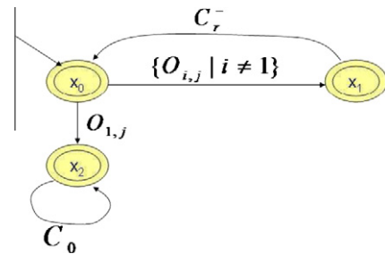
Fig. 15. Supervisor automaton S_f for the formation control.
