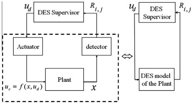
Fig. 22. Applying the discrete supervisor to the original plant.
