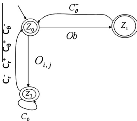
Fig. 19. Inter-collision avoidance supervisor.
