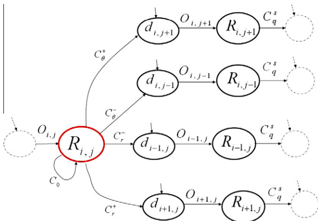
Fig. 11. DES model of the system with controllable and uncontrollable event sets \Sigma_c = \{C_r^+, C_r^-, C_\theta^+, C_\theta^-, C_0\} and \Sigma_{uc} = \{O_{ij} | 1 \leq i \leq n_r - 1, 1 \leq j \leq n_\theta - 1\} .
