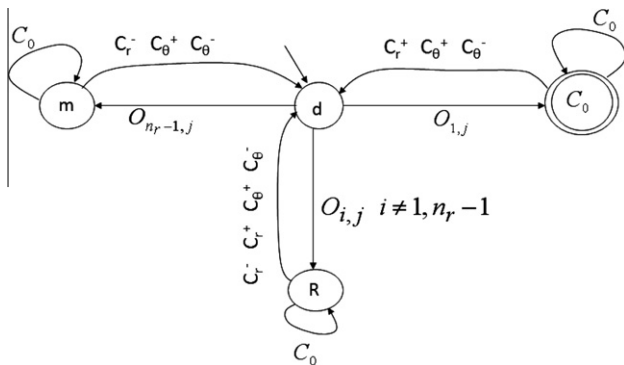
Fig. 12. Refined model of the plant G_{ref} .
