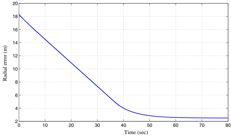
Fig. 25. Absolute distance from the desired position.
