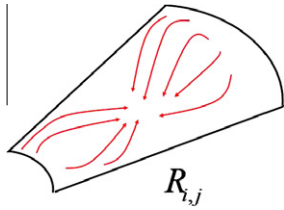
Fig. 7. Invariant region.
