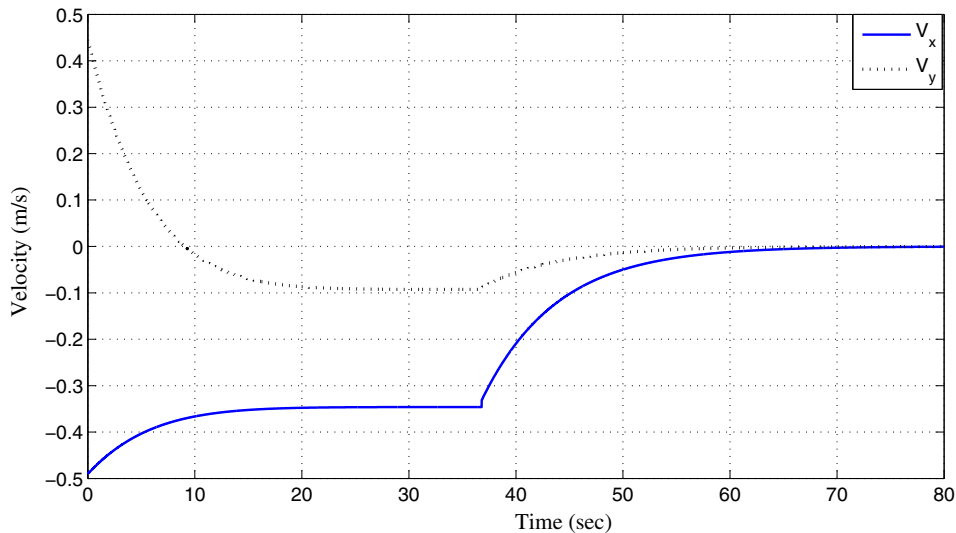
Fig. 24. Generated velocities V_x and V_y for an initial state inside the region R_{4,1} .
