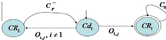
Fig. 16. The refined closed loop system.
